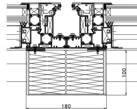
DETAIL CHENEAU
