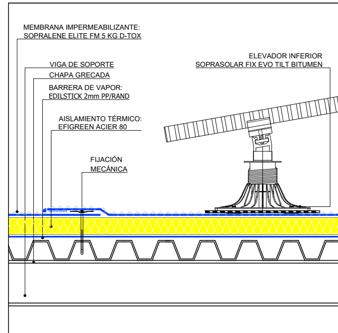
DETALLE SOPRASOLAR FIX EVO TILT
